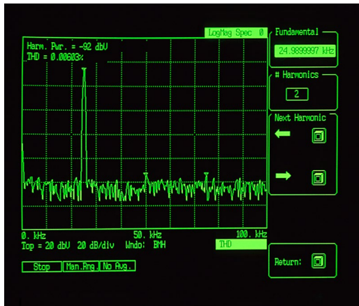
Spectrum analysis
