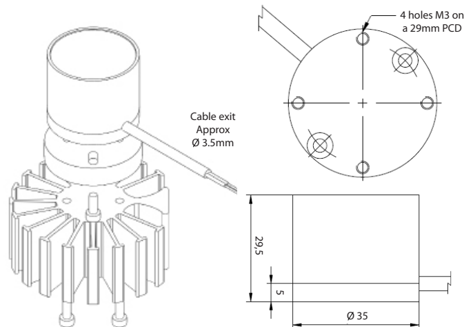
Area light heatsink adaptor included with Heatsink
