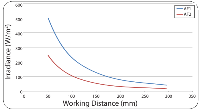
Figure 2 - Irradiance vs. working distance for AF1-630 (narrow beam) and AF2-630 (wide beam) measured at maximum operating current (current mode).
