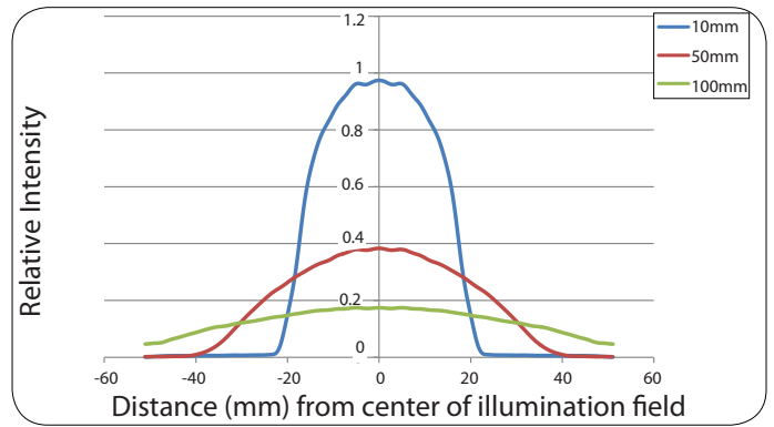
Figure 4 - Intensity profile for AF2-630. Working distances (WD) of 10, 50, and 100 mm.
