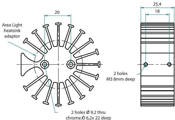
Area light heatsink adaptor included with Heatsink
