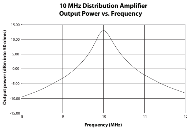
10 MHz distribution amplifier, output power vs. frequency
